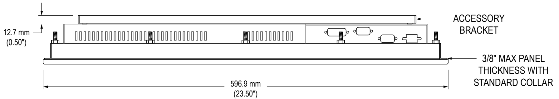
Bottom View
