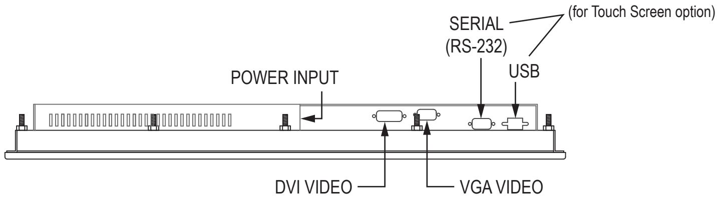
Bottom View
